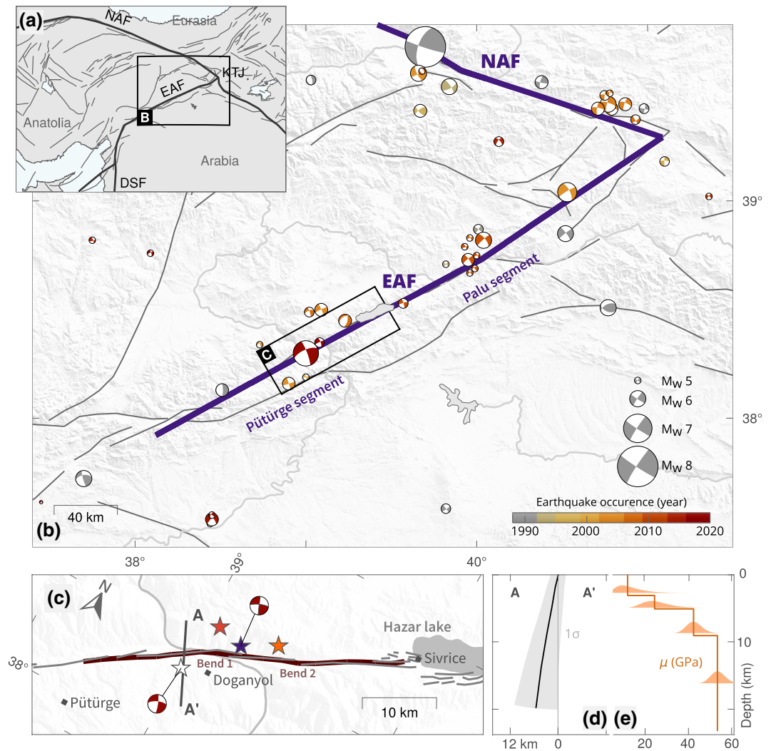
Figure 1. Tectonic setting and assumed characteristics for the Elazığ earthquake. (a) Tectonic setting of the area, plate boundaries are shown in thick black lines. East and North Anatolian Faults are labeled (EAF and NAF), as well as the Dead Sea fault (DSF) and Karhova Triple Junction (KTJ). (b) Active fault traces (Basilic et al., 2013) and seismicity since 1976 (GCMT, Dziewonski et al., 1981) around the EAF and NAF. The Elazığ earthquake focal mechanism (GCMT) is in red. (c) Details of assumed (dark red) and mapped (gray) fault trace at the surface. Two structural bends of the causative fault geometry are highlighted. Possible epicenters are shown with white, red, purple, and orange stars (from left to right on the map), respectively, from GCMT, Jamalreyhani et al. (2020) and KOERI and AFAD (2020). (d) Assumed fault geometry at depth and associated uncertainty (standard deviation of 5^\circ around the assumed dip and 1 km around the fault surface trace). (e) Assumed shear moduli with depth (derived from Maden, 2012; Ozer et al., 2019) and associated uncertainties.
