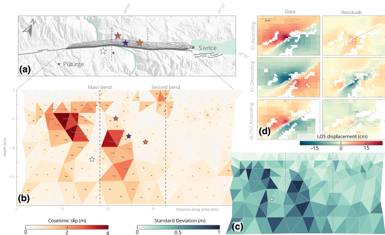
Figure 3. Inferred average slip model and associated posterior uncertainty for the Elaziğ earthquake. (a) Map view of the fault trace, subfaults contours at depth and local setting. Possible epicenters are shown with white, red, purple, and orange stars (from left to right on the map), respectively, from GCMT, Jamalreyhani et al. (2020) and KOERI and AFAD (2020). (b) Depth view of the average total slip amplitudes and directions. (c) Standard deviation of the inferred strike-slip parameters. (d) Observed and predicted surface displacement in the LOS direction from Sentinel-1 ascending and descending, and ALOS-2 ascending, InSAR.
